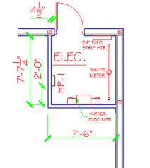
ENLARGED ELEC. RM. PLAN 1/4" = 1'-0"
